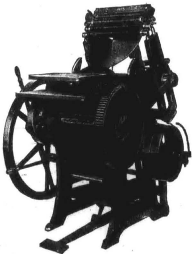
GORDON JOB PRESS. PRINTS SHEET 12 x 18
